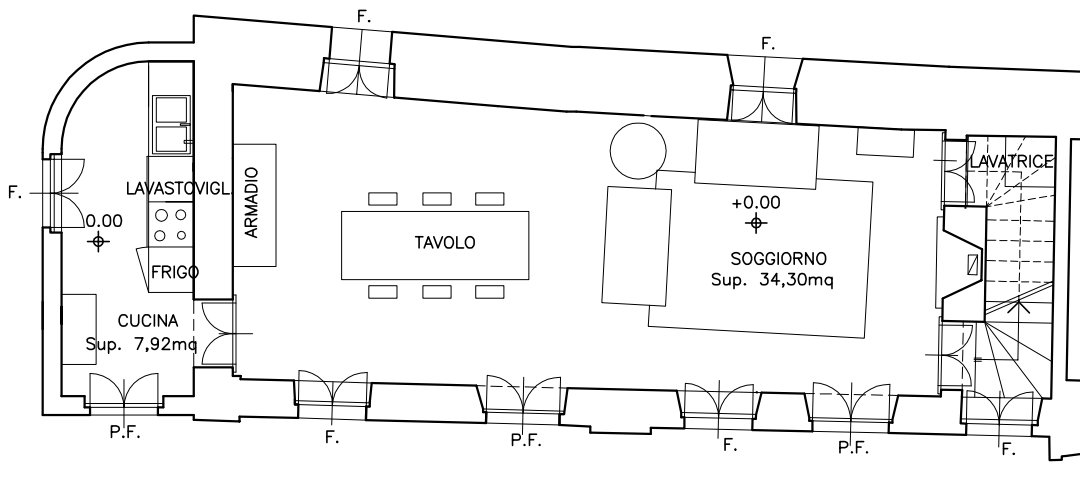
PIANO TERRA
